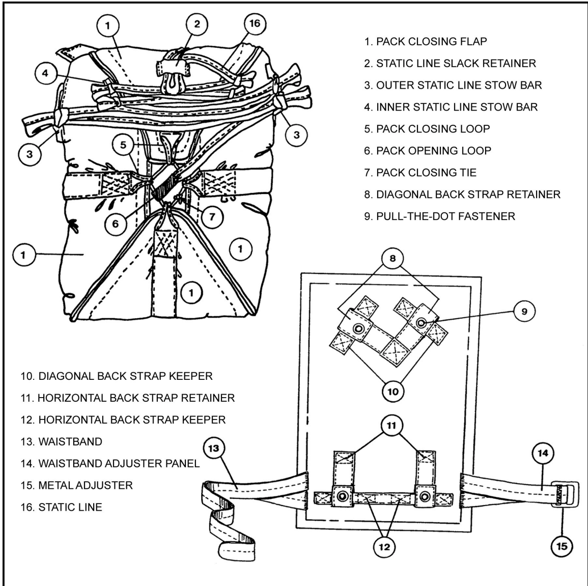
Figure 2-3. T-10C parachute pack tray and nomenclature.
