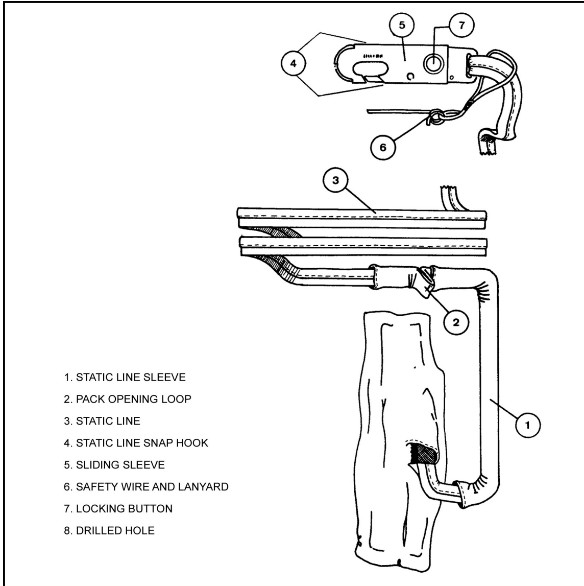
Figure 2-2. Static line and nomenclature.
