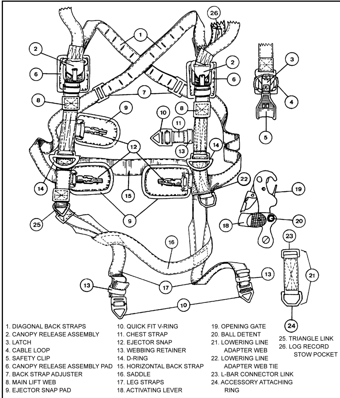
Figure 2-1. T-10C harness assembly and nomenclature.
