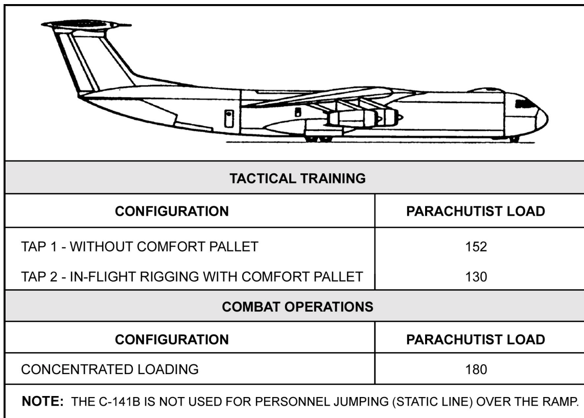
Figure 16-8. C-141B Starlifter.
