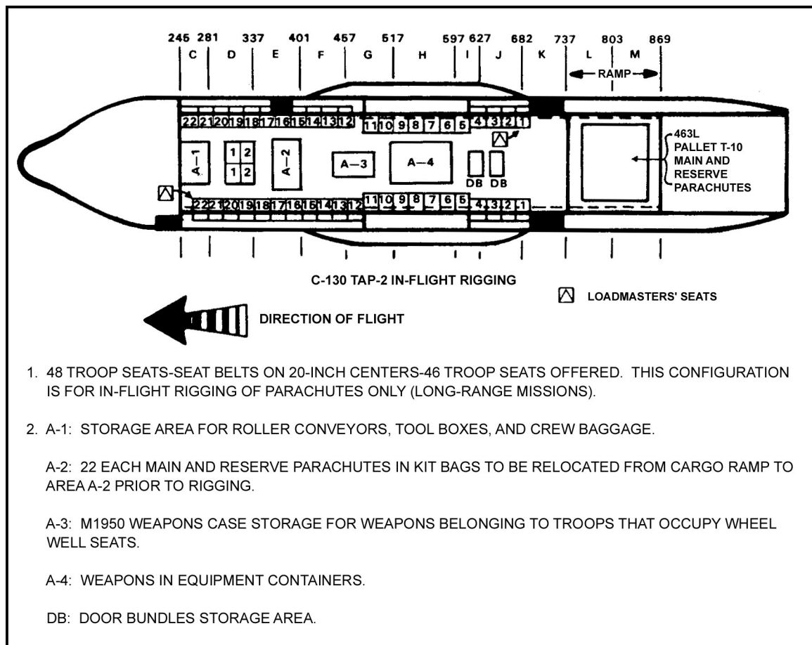
Figure 16-3. C-130 configuration for in-flight rigging (48 seats).
