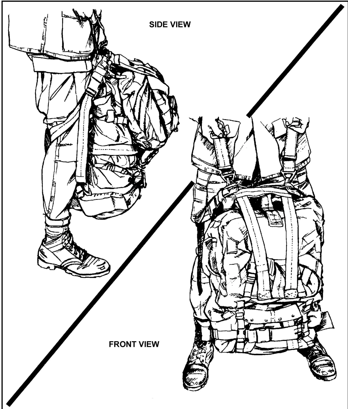
Figure 12-66. FPLIF with patrol pack attached to jumper.
