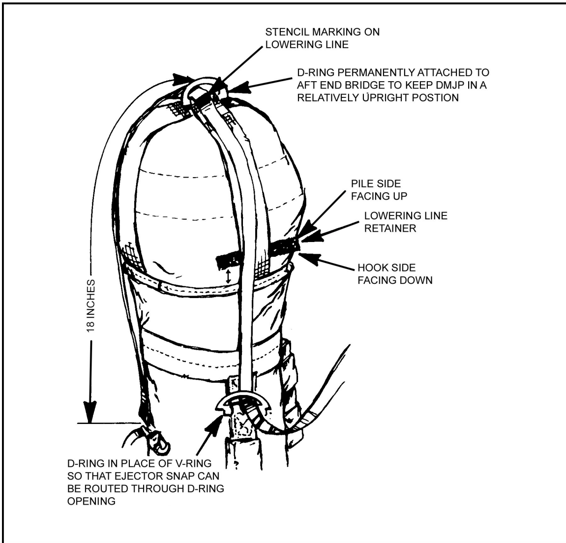
Figure 12-46. DMJP modified with D-ring.
