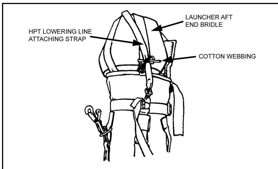
Figure 12-41. Lowering line attaching strap secured.
