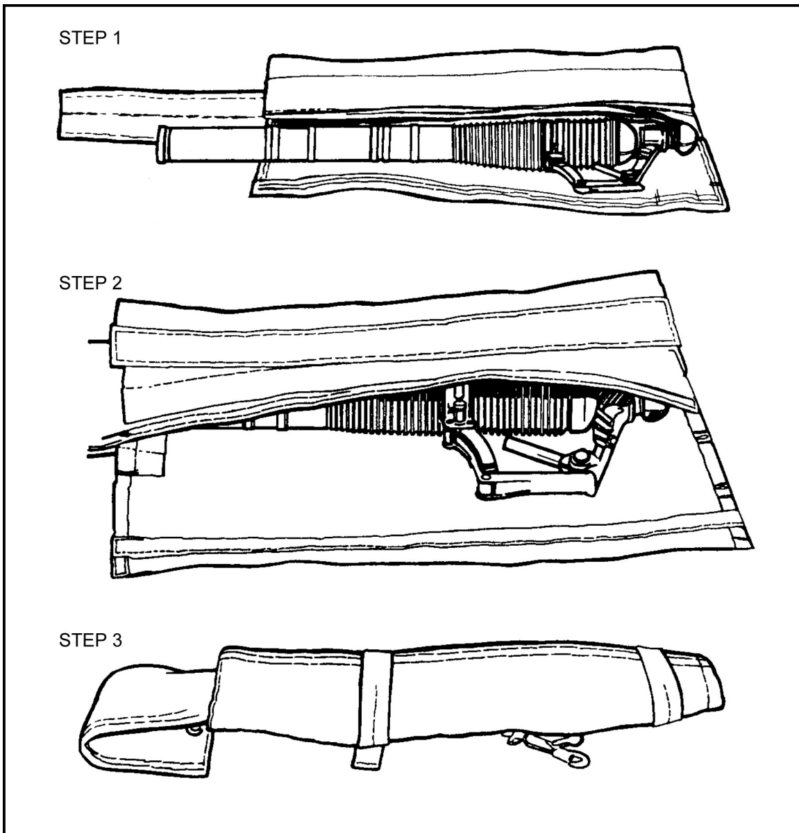
Figure 12-20. Barrel packed.
