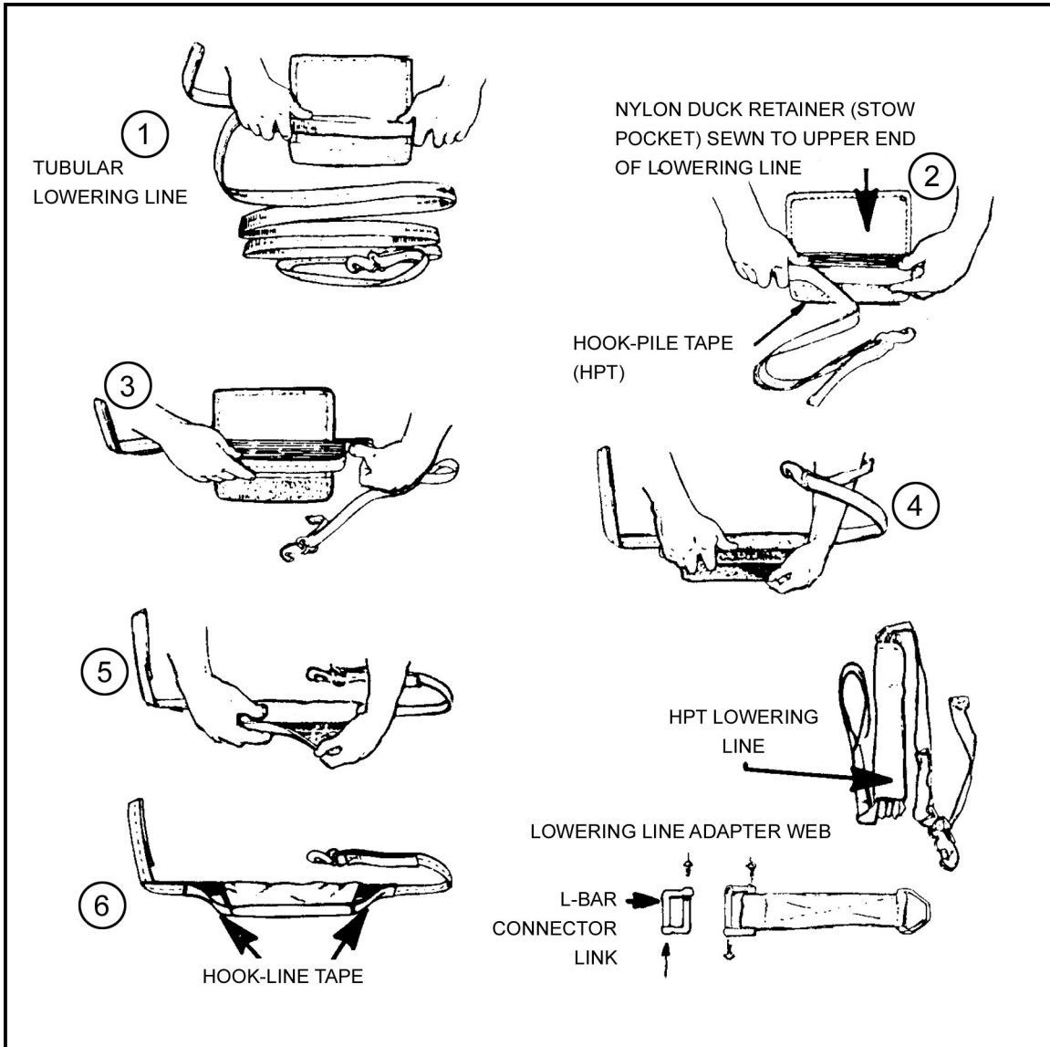
Figure 12-3. HPT lowering line.
