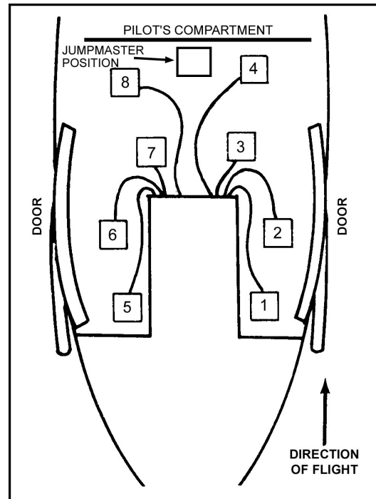
Figure 17-5. UH-1 seating configuration, overhead anchor line system.
