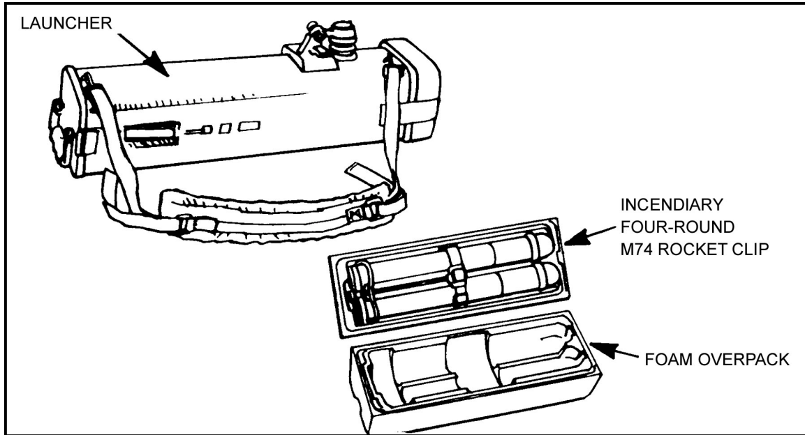
Figure 12-29. Launcher and rockets.
