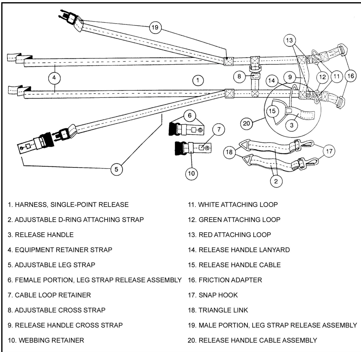
Figure 12-2. HSPR (NSN 1670-01-227-7992).
