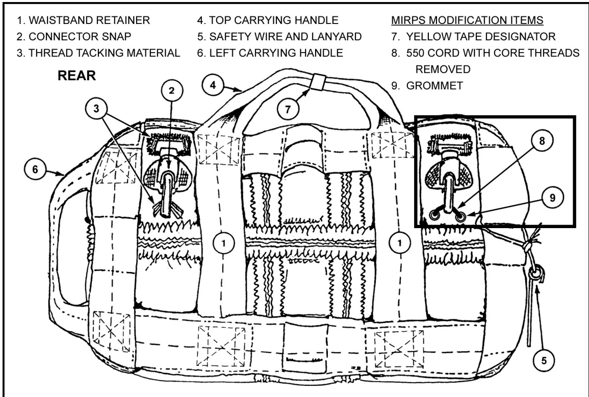
Figure 2-4. MIRPS/T-10 reserve parachute pack tray and nomenclature (back).
