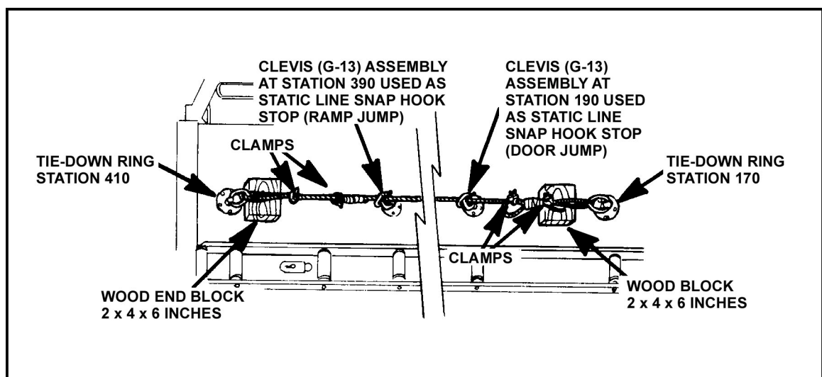
Figure 18-6. CH-46 anchor line cable installation.
