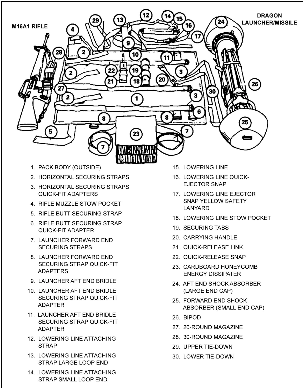
Figure 12-30. Nomenclature, DMJP.
