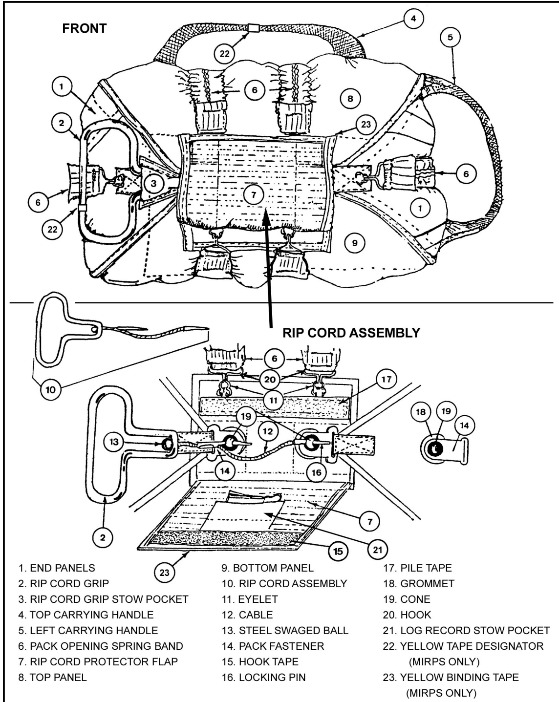
Figure 2-4. MIRPS/T-10 reserve parachute pack tray and nomenclature (front).
