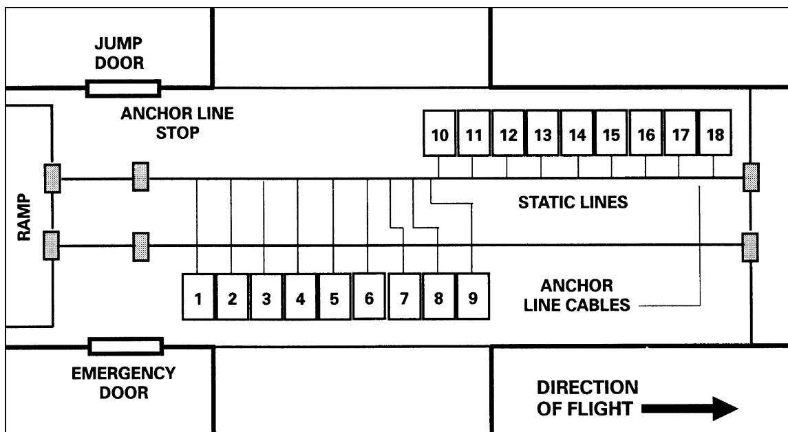
Figure 19-5. C-23B seating configuration.
